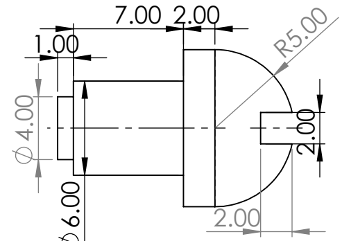
Oval Fillister
