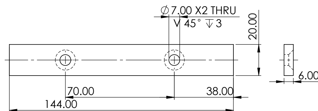
Base Plate
