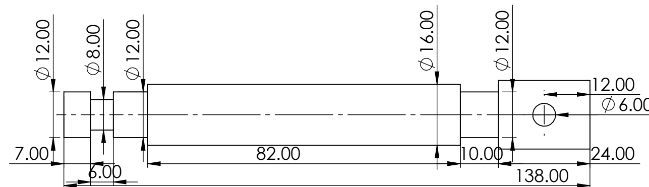
Jaw Screw
