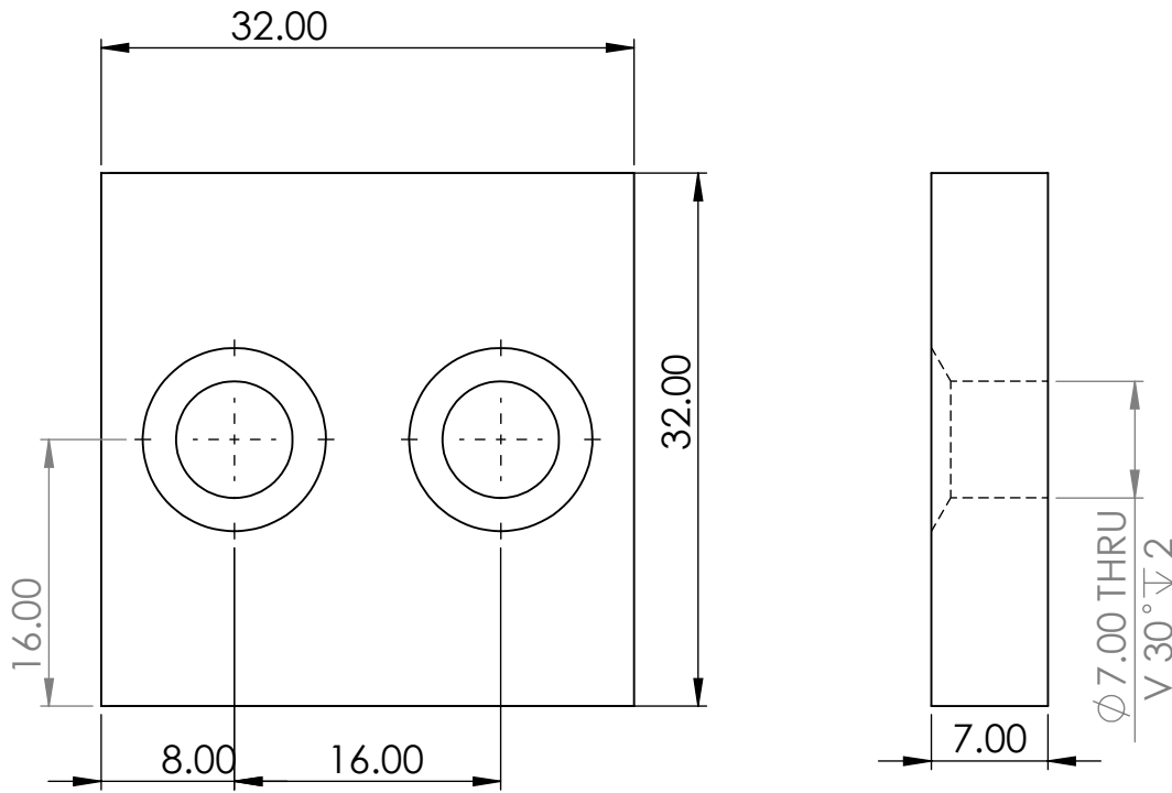
Clamping Plate
